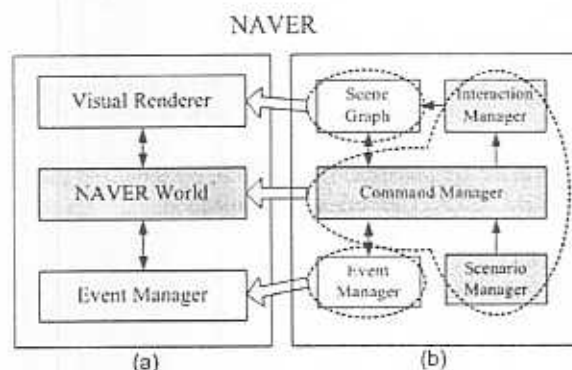
Fig.3. NAVER architecture; (a) conceptual components of NAVER in CIVE (b) components of NAVER
