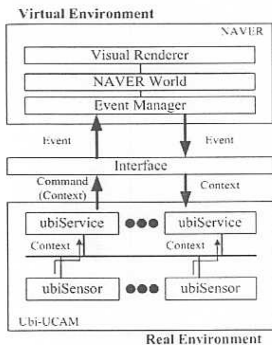
Fig. 1. Architecture of CIVE
