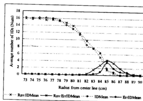
Fig. 5 Experimental results of the filtering method. The error occurs at the edge of sensing area. And the size of error occurring is reduced by the filtering method.
