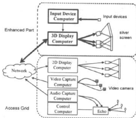
Fig. 1 The picture of e-AG system
