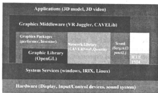
Fig. 2 Software structure of e-AG
