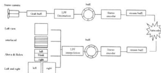
Fig. 3 Off-line process
