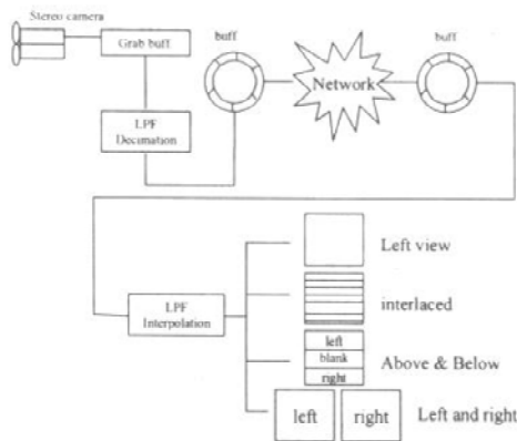
Fig. 4 On-line processing
