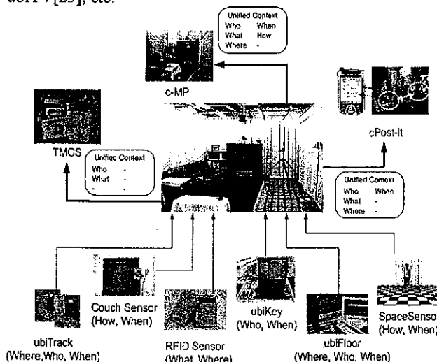
Figure 12: Example of Sensors and Services based on Unified User-centric Context
