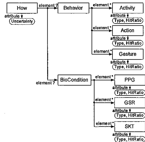
Figure 5: 'How' Element Modeling
