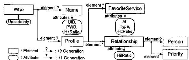
Figure 1: 'Who' Element Modeling
