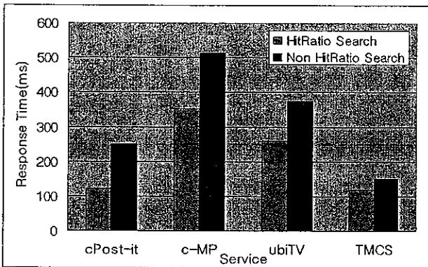
Figure 14: Comparison of average response time between 'HitRatio' search-based and non-'HitRatio' search-based service.
