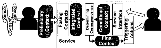
Figure 7: Unified Context: Preliminary, Integrated, Final, and Conditional Context
