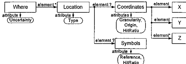
Figure 2: 'Where' Element Modeling
