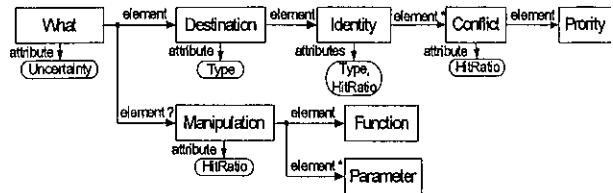
Figure 4: 'What' Element Modeling
