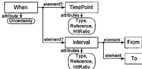
Figure 3: 'When' Element Modeling
