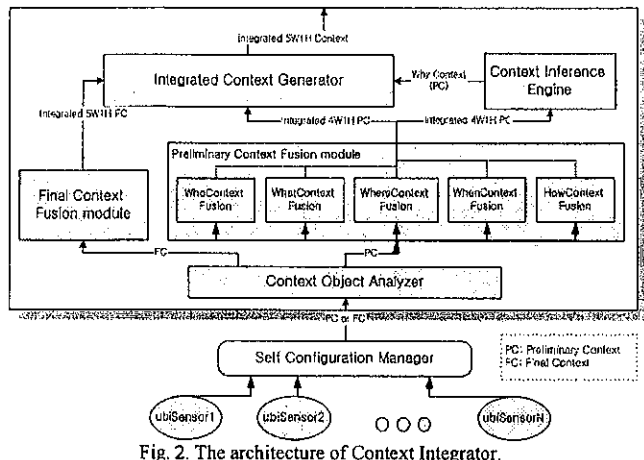
Fig. 2. The architecture of Context Integrator.
