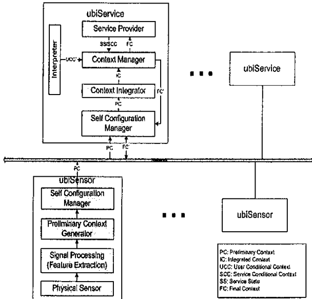
Fig. 1. The architecture of ubi-UCAM 2.0.
