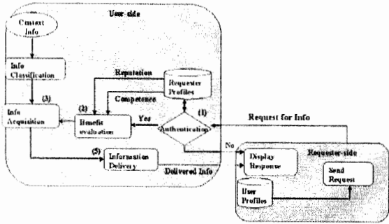
Fig. 2. Personal Information Disclosure Control Mechanism
