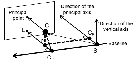
Fig. 7. Orthogonal projection of camera centers
