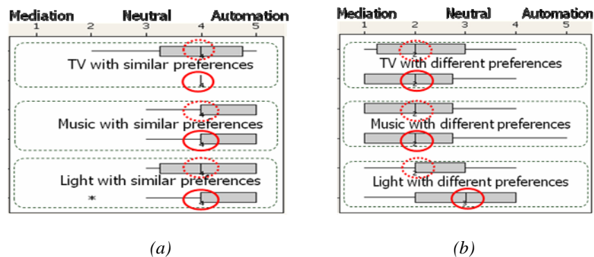
Figure 13: Box plots of participants' preferred resolution method in internal conflicts from an application involving similar preferences(a) and different preferences(b).
