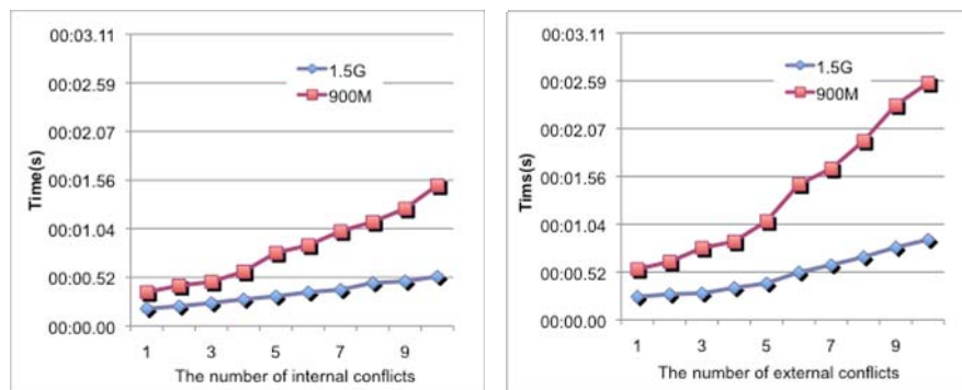
Figure 12: Time spent on reasoning service conflicts involving internal conflicts (a) and external conflicts (b).
