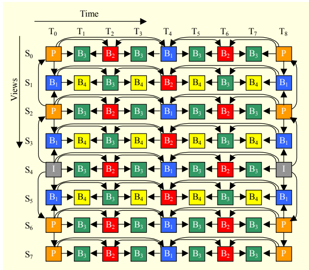
Fig. 7. Proposed MVC scheme based on JMVM.
