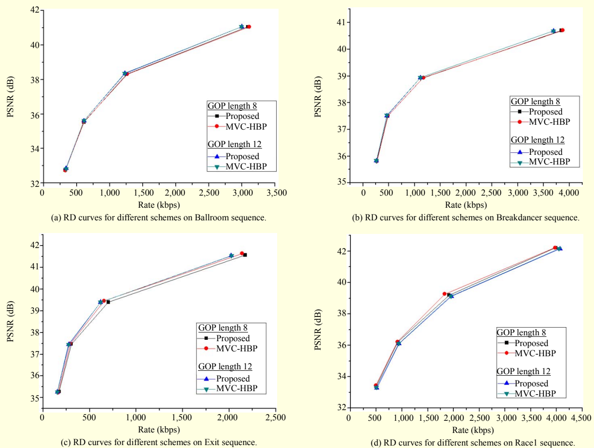
Fig. 8. RD performances for different schemes with same GOP size.
