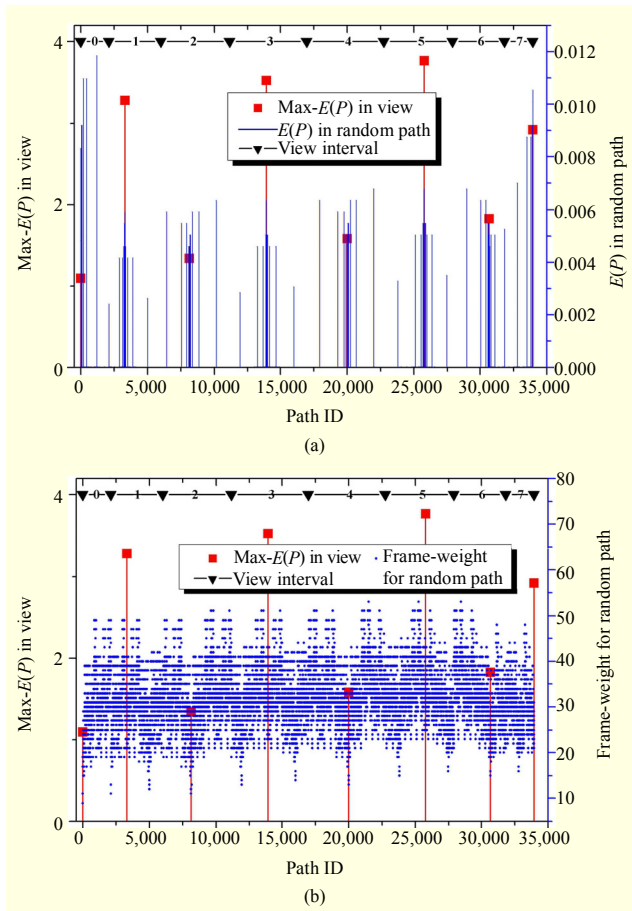
Fig. 5. (a) Comparative results of \max-E(P) in view and E(P) in P for MVC-HBP random graph model and (b) comparative results of \max-E(P) in view and W(P) for P for MVC-HBP random graph model.
