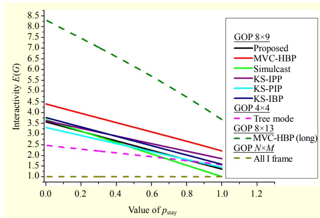
Fig. 2. Values of E(G) for different MVC schemes when different values of p_{state_i} are selected.
