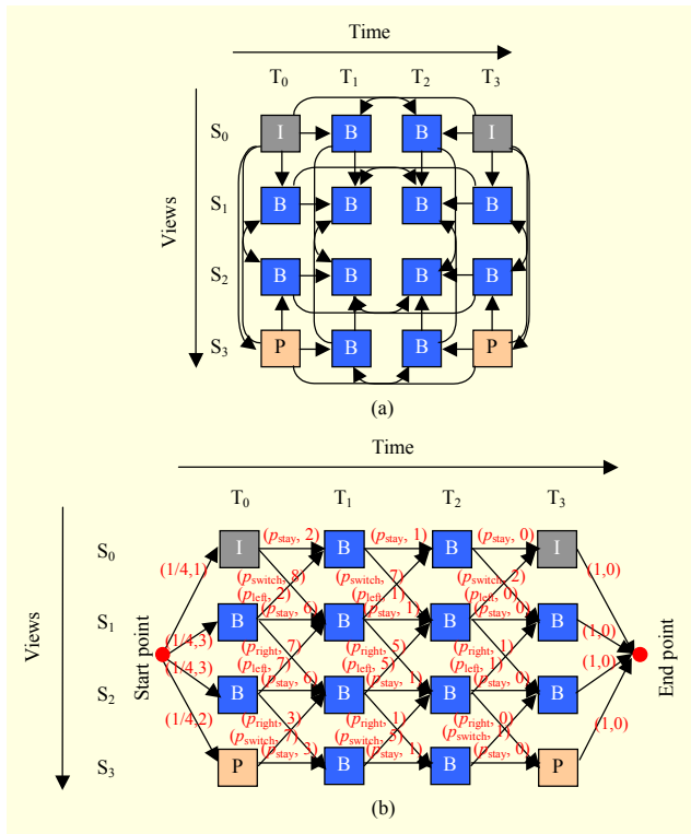
Fig. 1. (a) Multiview video coding sample scheme 1 and (b) weighted random graph model G for sample scheme 1.
