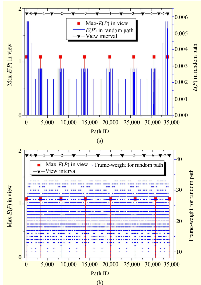
Fig. 6. (a) Comparative results of \max-E(P) in view and E(P) in P for Simulcast random graph model and (b) comparative results of \max-E(P) in view and W(P) for P for Simulcast random graph model.
