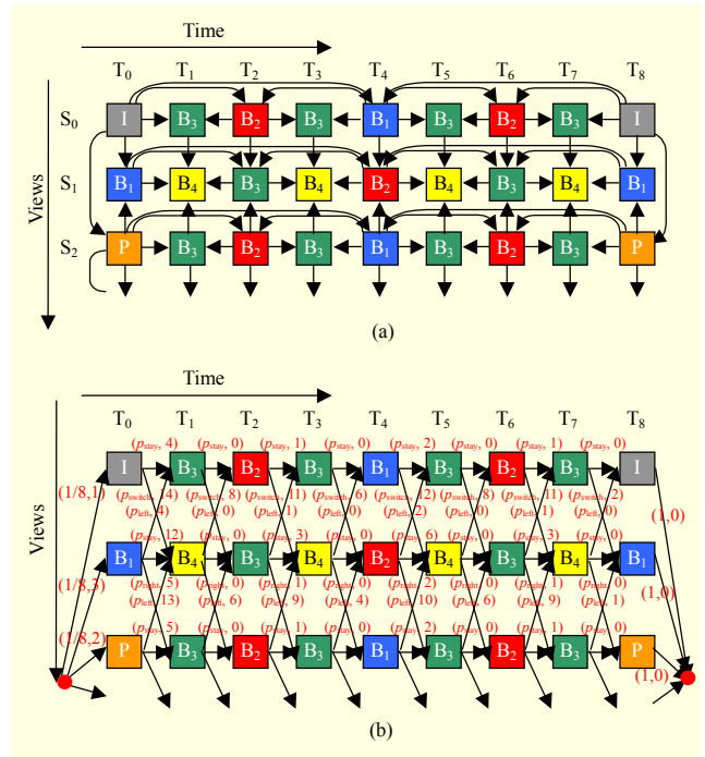
Fig. 4. (a) MVC-HBP scheme in JMVM prediction structures and (b) weighted random graph model G for the JMVM prediction structure in (a).
