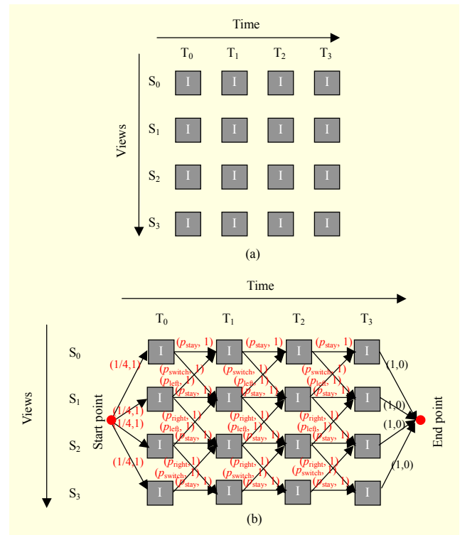
Fig. 3. (a) MVC sample scheme 2 and (b) weighted random graph model G for sample scheme 2.
